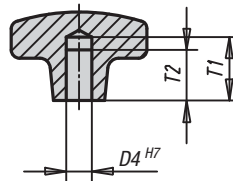
Form C Sackloch
