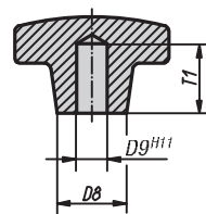
Form G Sackloch
